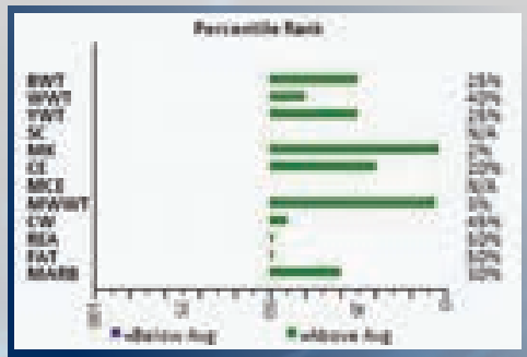
CML 216K - EPD Chart
